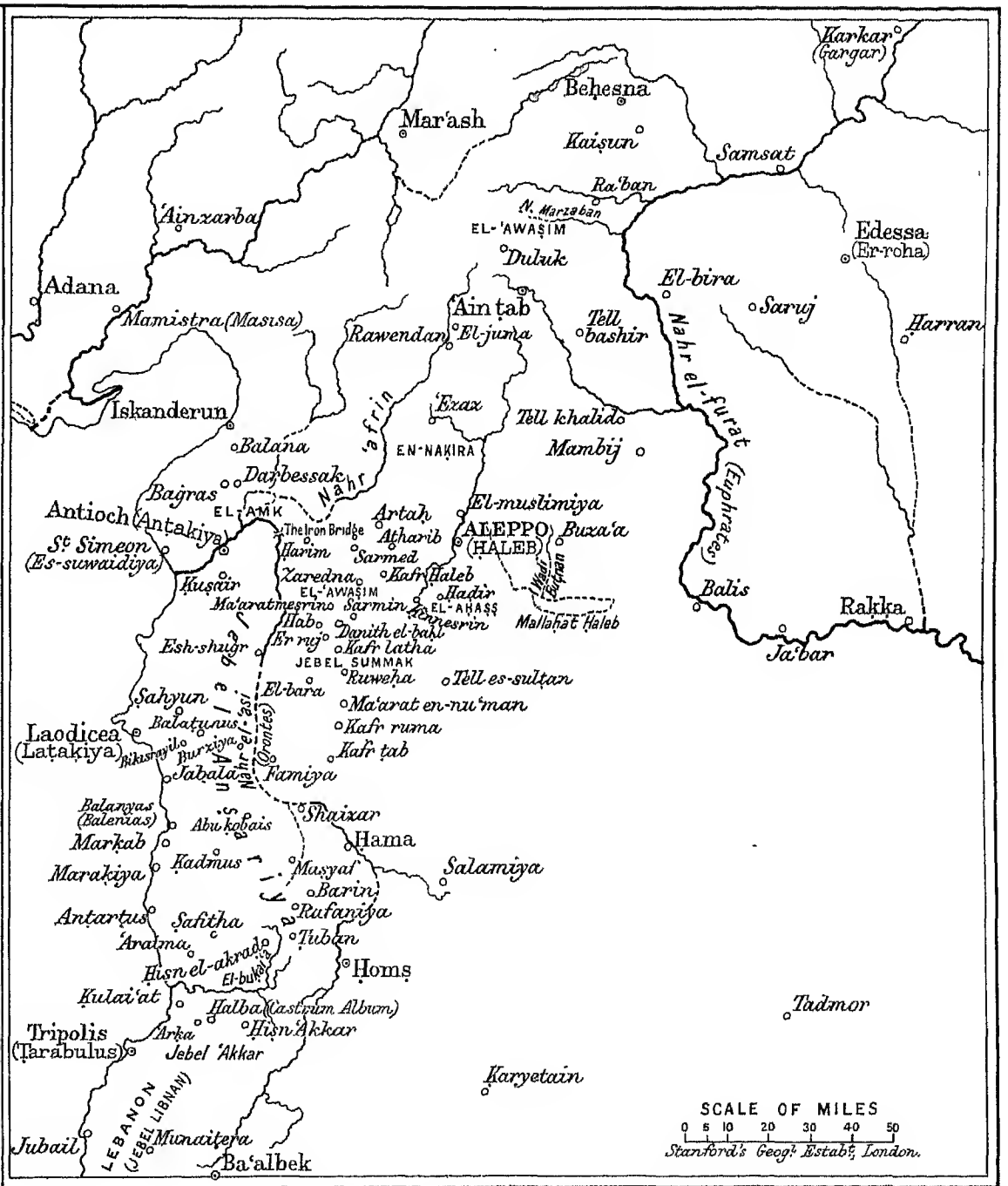
NORTHERN SYRIA AND EUPHRATESIA.
